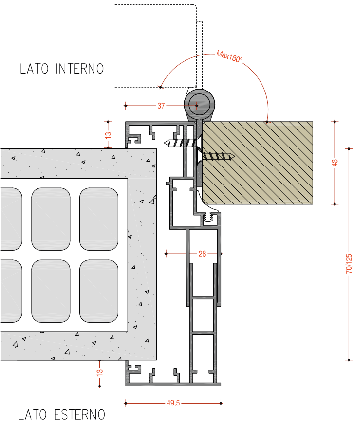
NOVA GHIBLI 50 MINIMAL
